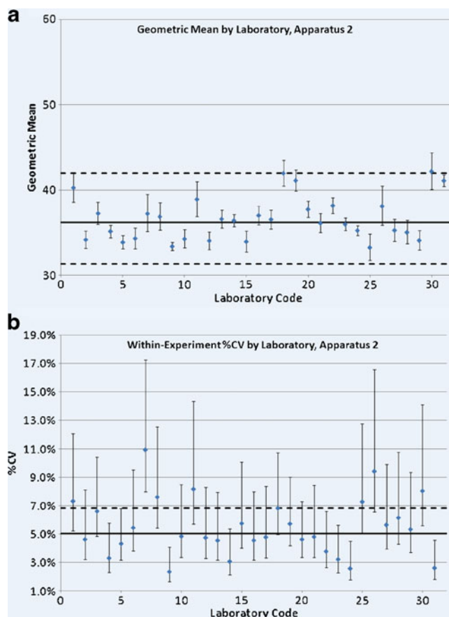
Fig. 5 GM and %CV by Laboratory, Apparatus 2. Error bars are 95% confidence intervals based on each laboratory's between-position variability. Horizontal lines are the combined value from the collaborative study and the single-stage Lot P1 PVT limits for an instrument with six positions. Limits for seven- and eight-position instruments are tighter. The limits for the geometric mean are those at the time of the collaborative study
